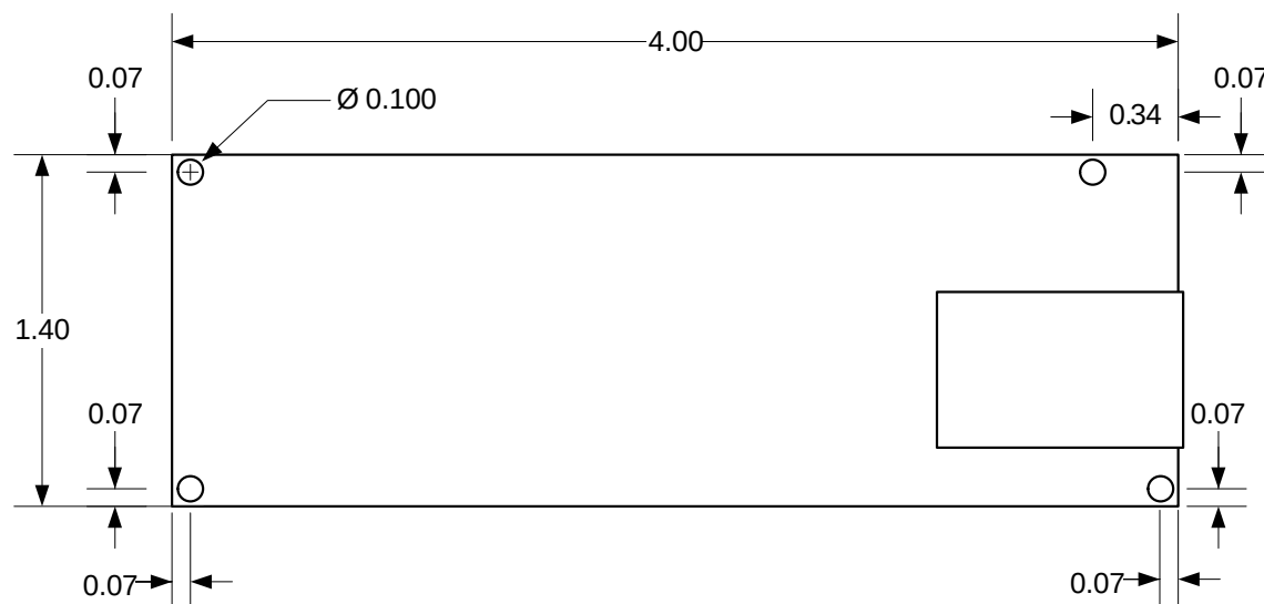
Figure B-3. EK-LM3S9D92 Evaluation Board Dimensions
