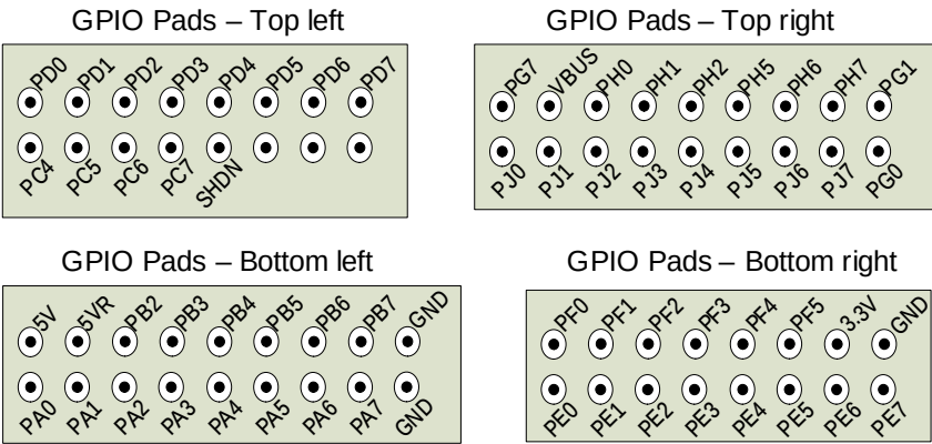
Figure 2-2. GPIO Pads
