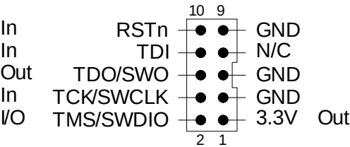
Figure 2-3. JTAG/SWD Connector
