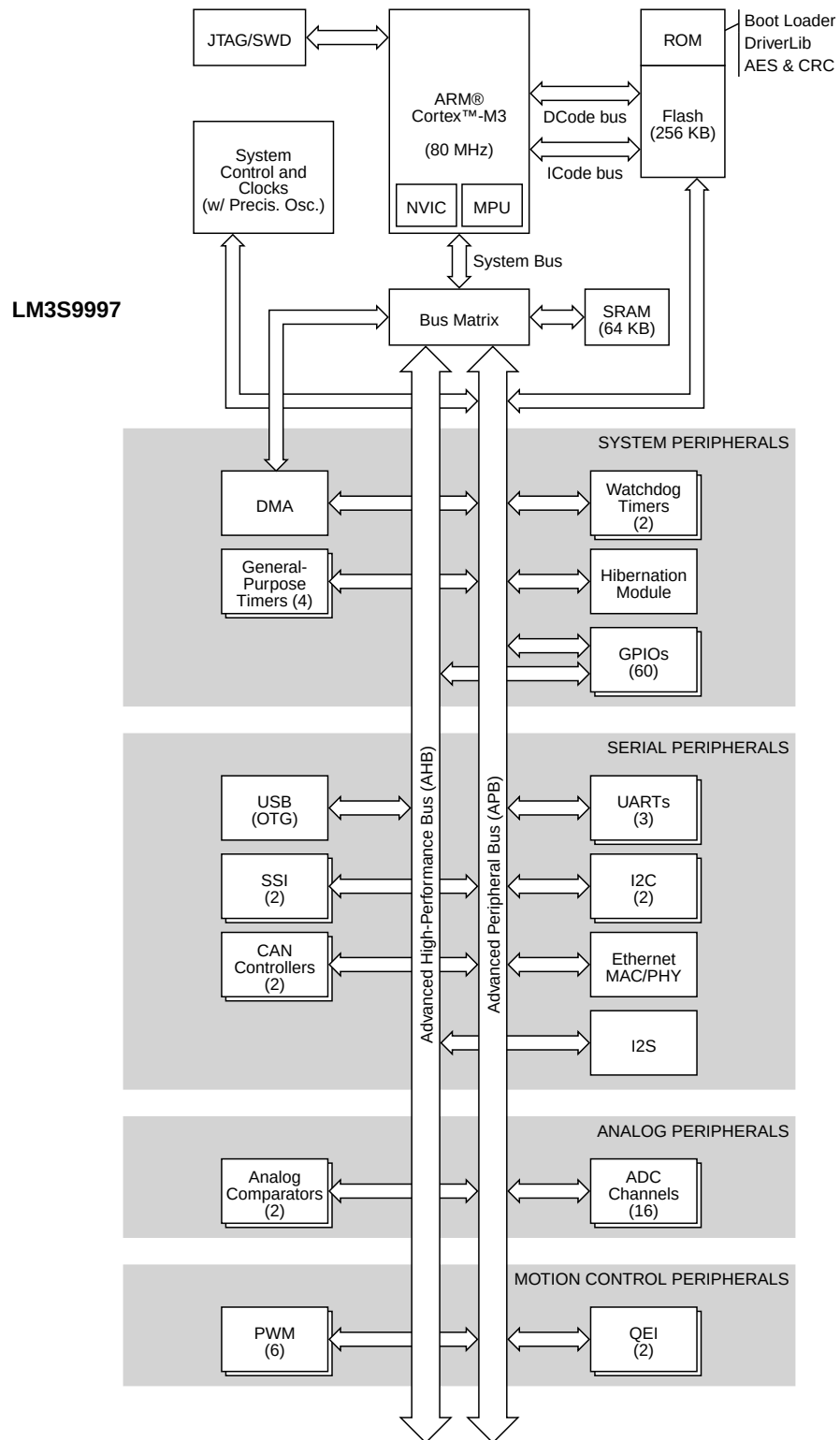
Figure 1-1. Stellaris® LM3S9997 Microcontroller High-Level Block Diagram
