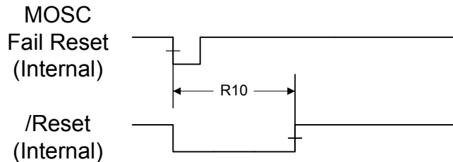
Figure 27-9. MOSC Failure Reset Timing
