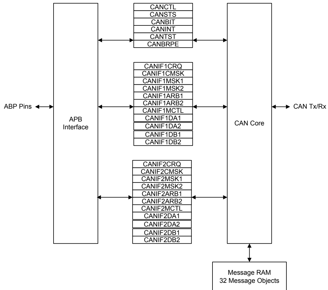
Figure 15-1. CAN Module Block Diagram
