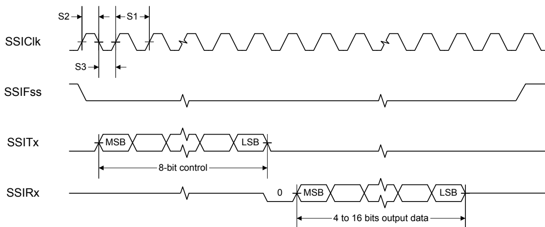
Figure 20-6. SSI Timing for MICROWIRE Frame Format (FRF=10), Single Transfer
