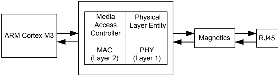
Figure 15-1. Ethernet Controller
