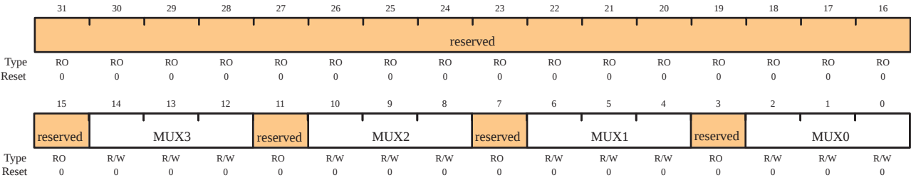
ADC Sample Sequence Input Multiplexer Select 2 (ADCSSMUX2)
