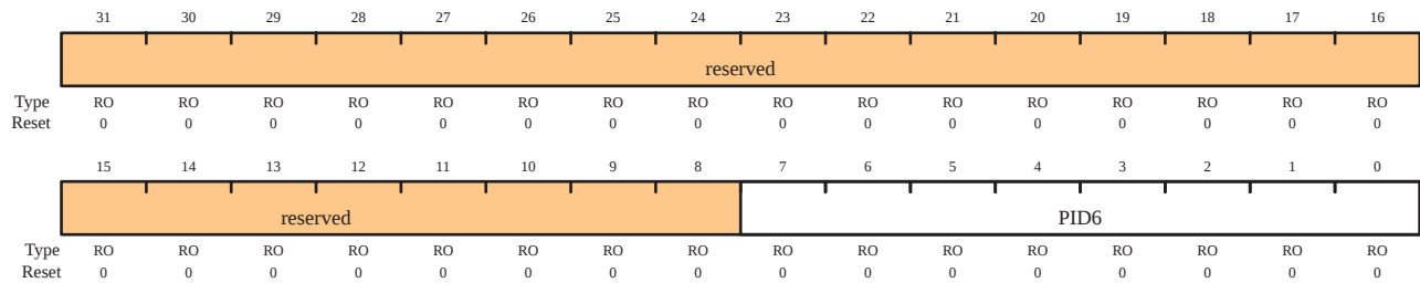
GPIO Peripheral Identification 6 (GPIOPeriphID6) Offset 0xFD8
