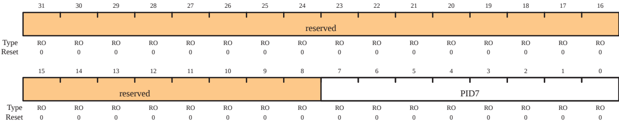
GPIO Peripheral Identification 7 (GPIOPeriphID7)
