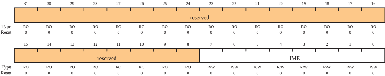
GPIO Interrupt Mask (GPIOIM) Offset 0x410
