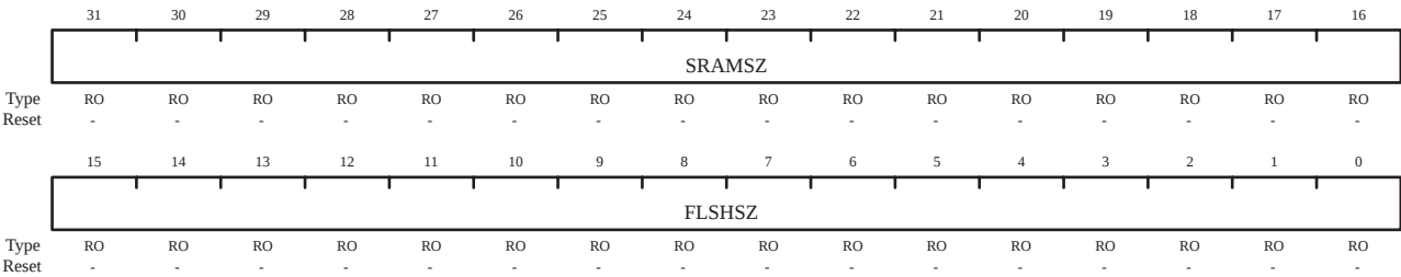
Device Capabilities Register 0 (DC0)
