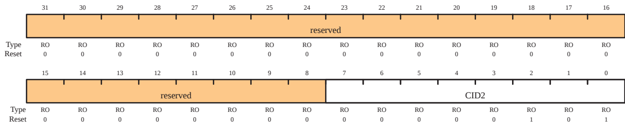
GPIO Primecell Identification 2 (GPIOCellID2) Offset 0xFF8
