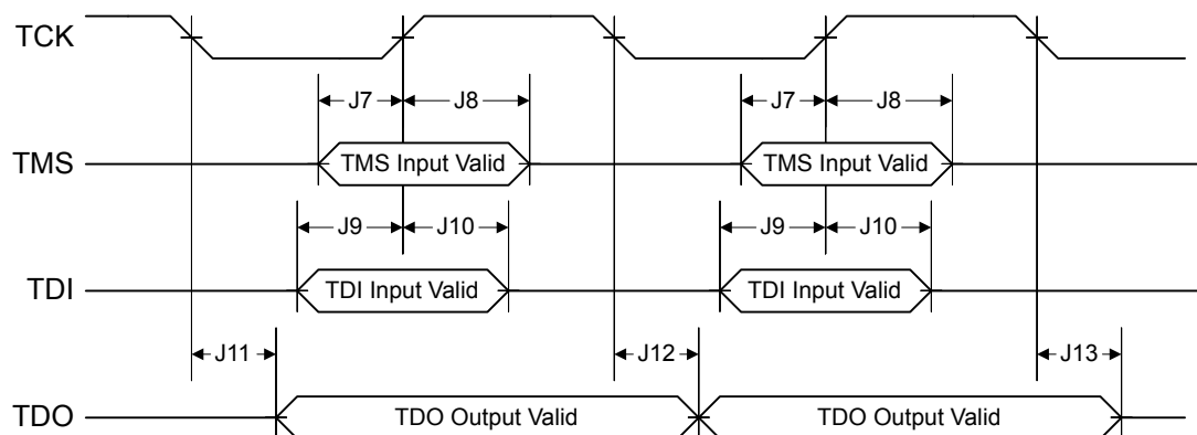
Figure 24-8. JTAG Test Access Port (TAP) Timing
