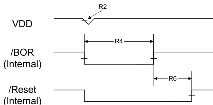
Figure 24-12. Software Reset Timing
