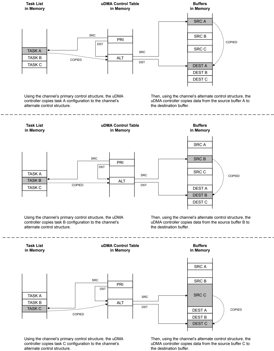
Figure 9-4. Memory Scatter-Gather, \mu DMA Copy Sequence
