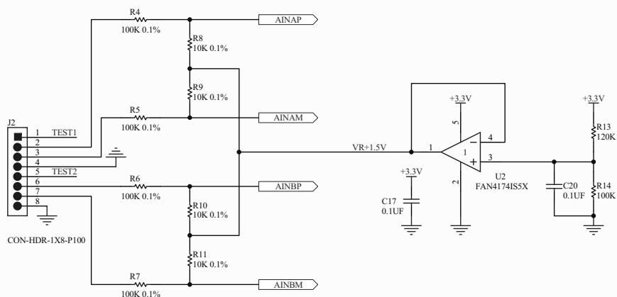
2 Channel Oscilloscope
