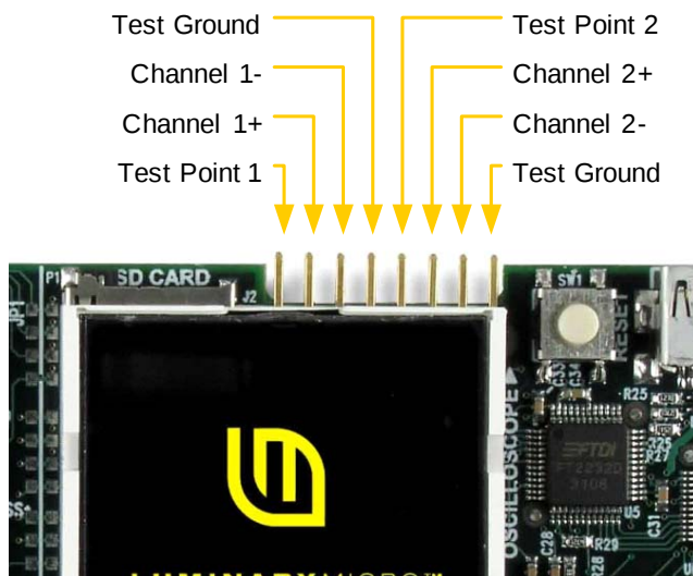
Figure 2-2. Oscilloscope Connections
