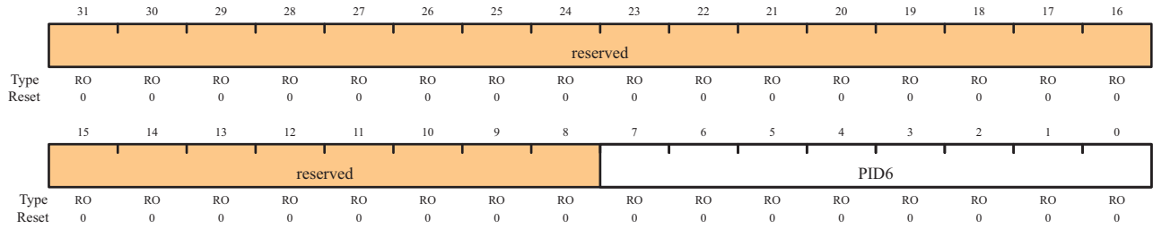
SSI Peripheral Identification 6 (SSIPeriphID6)
