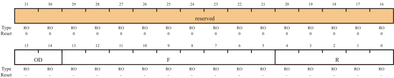
XTAL to PLL Translation (PLLCFG) Offset 0x064
