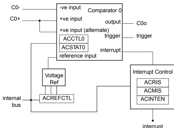
Figure 14-1. Analog Comparator Module Block Diagram
