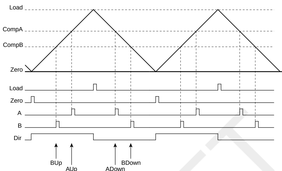
Figure 16-3. PWM Count-Up/Down Mode
