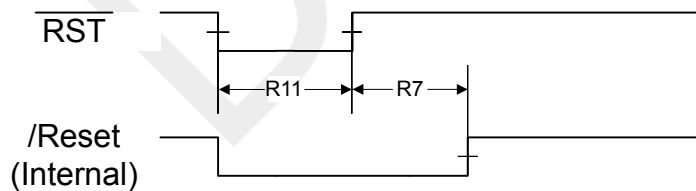
Figure 21-10. External Reset Timing (RST)
