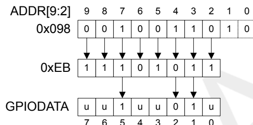
Figure 9-1. GPIODATA Write Example
