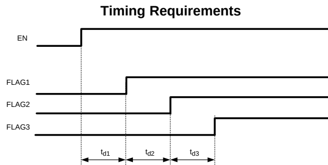
Figure 2. Power-Up Sequence
