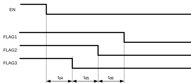
Figure 3. Power-Down Sequence
