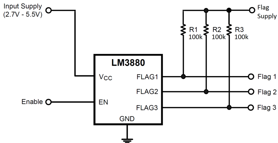
Figure 18. Sequencing Using Independent Flag Supply
