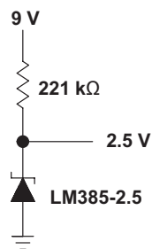
Figure 8. Reference From a 9-V Battery
