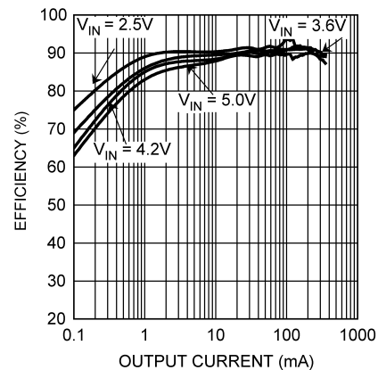
Figure 2. Efficiency vs. Output Current ( V_{OUT} = 1.8V )
