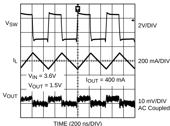
Figure 18. PWM Operation
