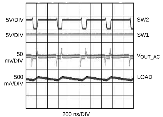
Figure 36. Typical Switching Waveform in Boost Mode (PWM Mode) V_{IN} = 3\text{ V} , V_{OUT} = 3.4\text{ V} , Load = 500 mA
