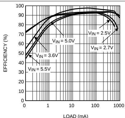
Figure 13. Efficiency at V_{OUT} = 3.4\text{ V} (Auto Mode)
