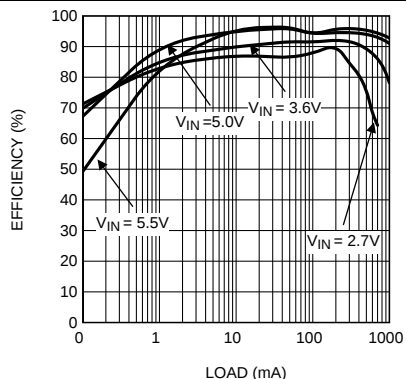
Figure 17. Efficiency at V_{OUT} = 5\text{ V} (Auto Mode)
