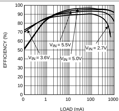
Figure 15. Efficiency at V_{OUT} = 4.5\text{ V} (Auto Mode)
