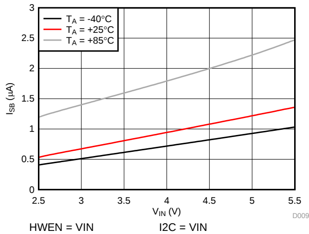
Figure 18. Standby Current vs Input Voltage
