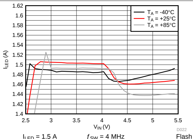
Figure 9. LED2 Current vs Input Voltage
