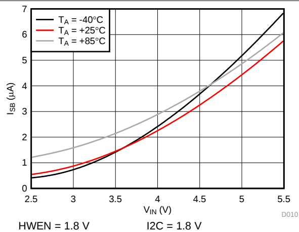
Figure 18. Standby Current vs Input Voltage
