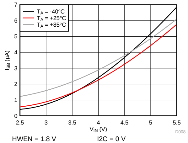
Figure 19. Standby Current vs Input Voltage
