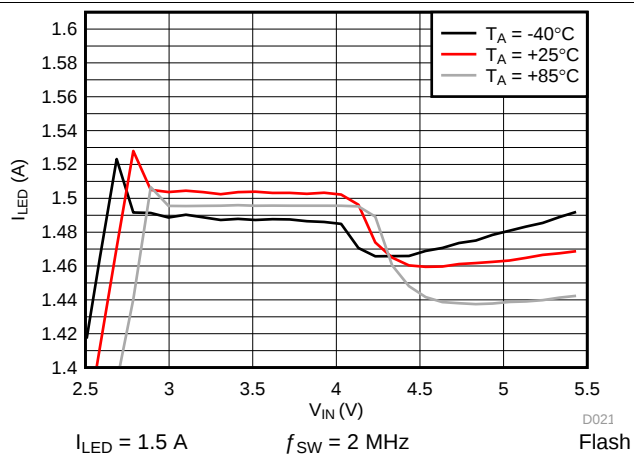
Figure 8. LED2 Current vs Input Voltage
