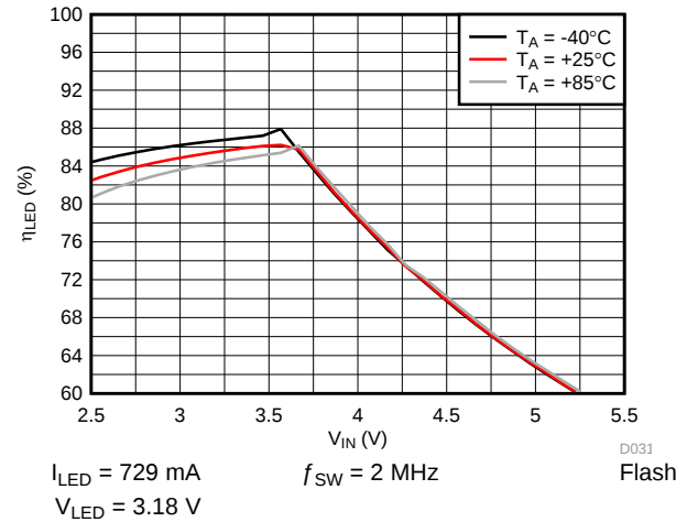
Figure 42. LED Efficiency vs Input Voltage
