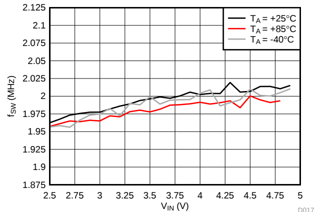
Figure 25. 2-MHz Switching Frequency vs Input Voltage
