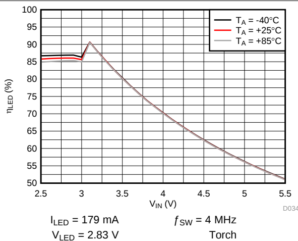
Figure 45. LED Efficiency vs Input Voltage
