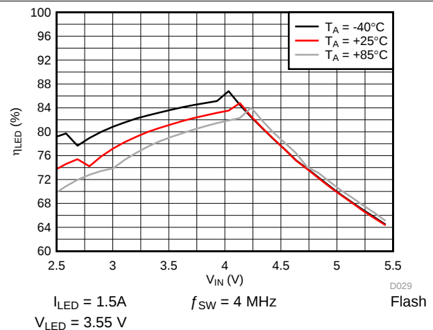
Figure 40. LED Efficiency vs Input Voltage
