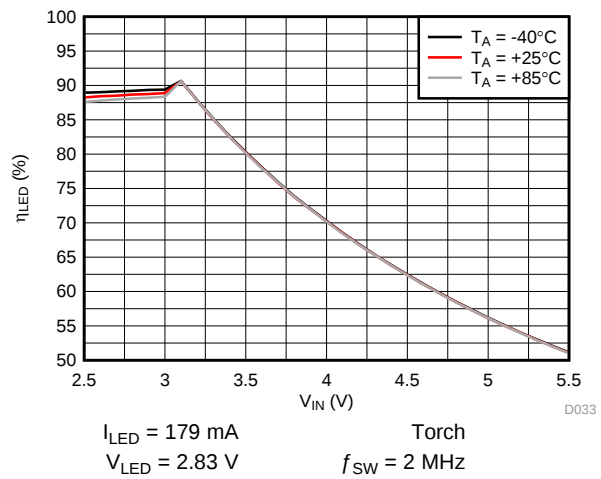
Figure 44. LED Efficiency vs Input Voltage
