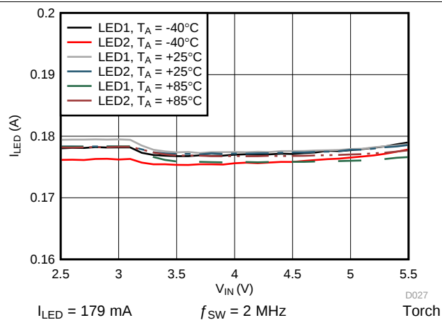
Figure 14. LED Current vs Input Voltage
