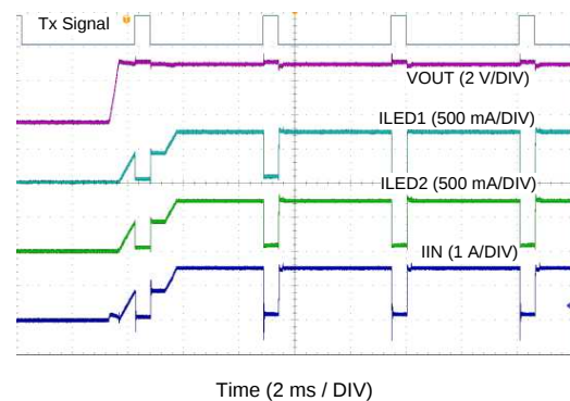
Figure 48. Start-Up
