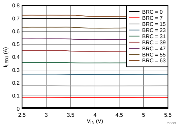
Figure 6. LED1 Current vs Input Voltage
