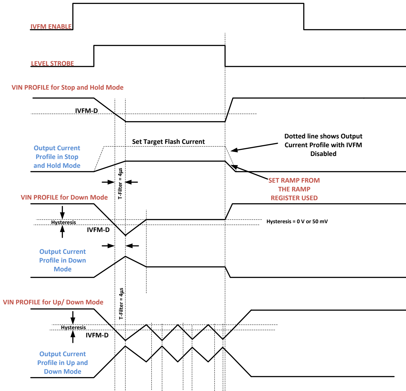
Figure 30. IVFM Modes
