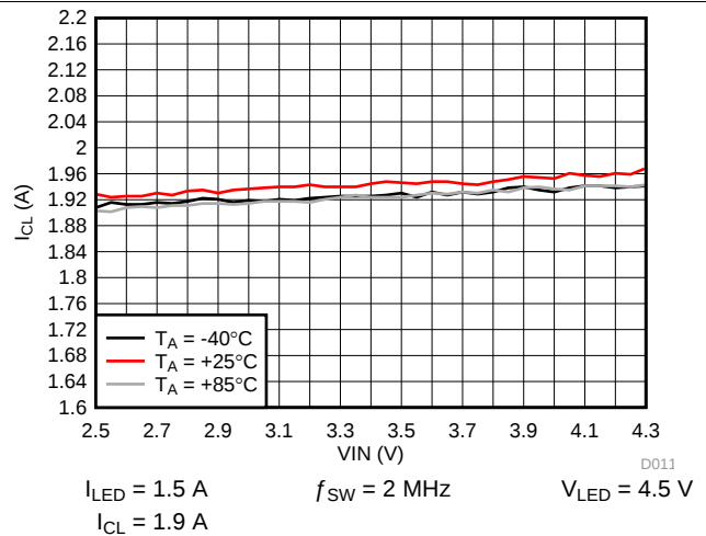
Figure 21. Inductor Current Limit vs Input Voltage
