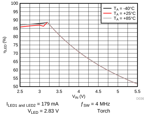
Figure 47. LED Efficiency vs Input Voltage
