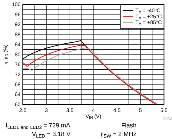
Figure 43. LED Efficiency vs Input Voltage
