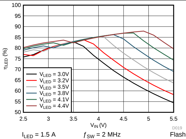
Figure 37. 2-MHz LED Efficiency vs Input Voltage
