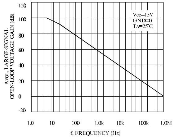
Figure 2. Open-Loop Frequency
