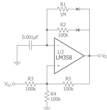
Figure 18. Pulse Generator
