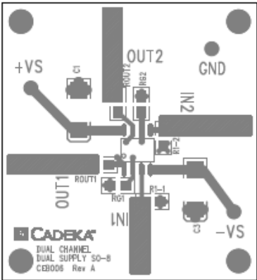
Figure 8. CEB006 Top View
