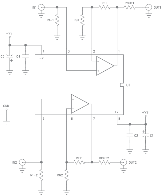
Figure 7. CEB006 Schematic
