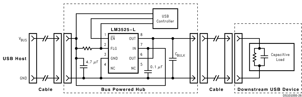
FIGURE 4. Soft-Start Application
