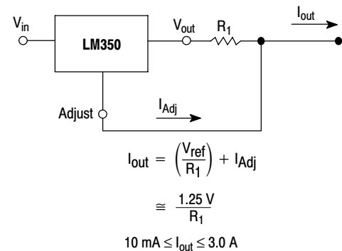
Figure 25. Current Regulator
