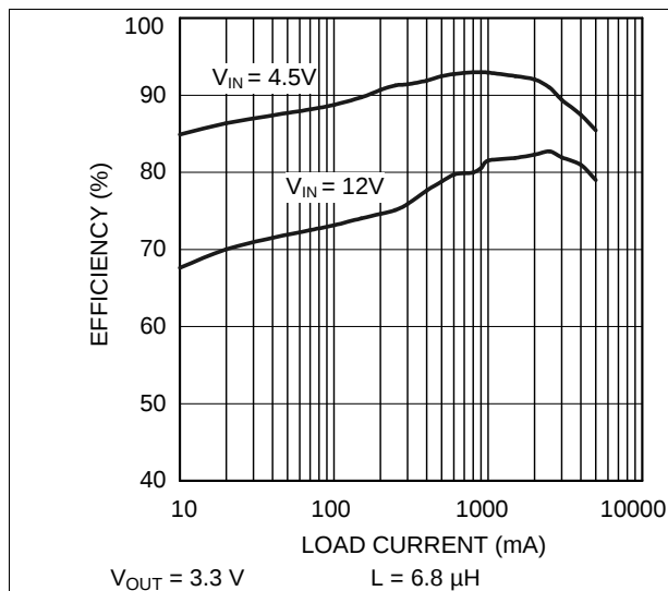
Figure 28. Efficiency vs Load Current
