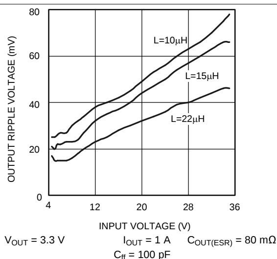
Figure 29. Output Ripple Voltage vs Input Voltage
