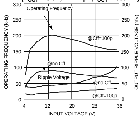
Feed-Forward Capacitor ( C_{ff} ) Effect ( V_{OUT} = 3.3\text{V} , L = 22\mu\text{H} , I_{OUT} = 500\text{mA} )
