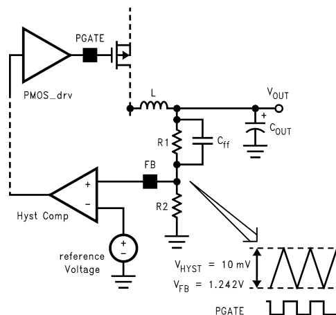
Figure 2. Hysteretic Window
