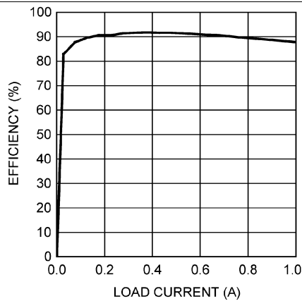
Figure 5. Efficiency vs. Load Current ( 3.3\text{ V}_{IN} and 12\text{ V}_{OUT} )
