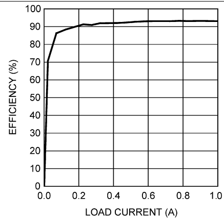
Figure 6. Efficiency vs. Load Current ( 5\text{ V}_{IN} and 12\text{ V}_{OUT} )
