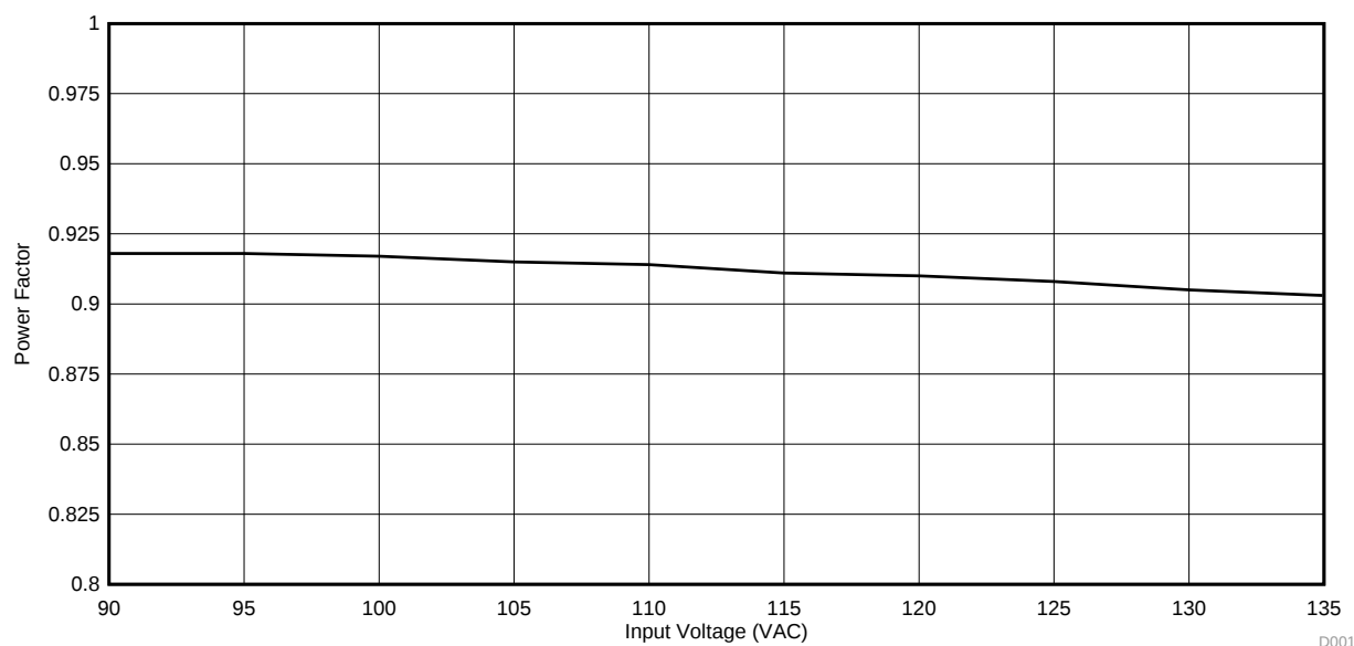
Figure 3. LM3445EVM-695 Power Factor
