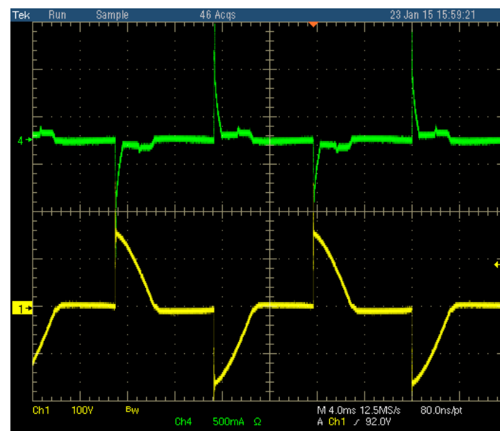
Figure 12. Lutron Leading Edge DVLV-6006, Output = 20 mA, V_{LED} = 22 V
