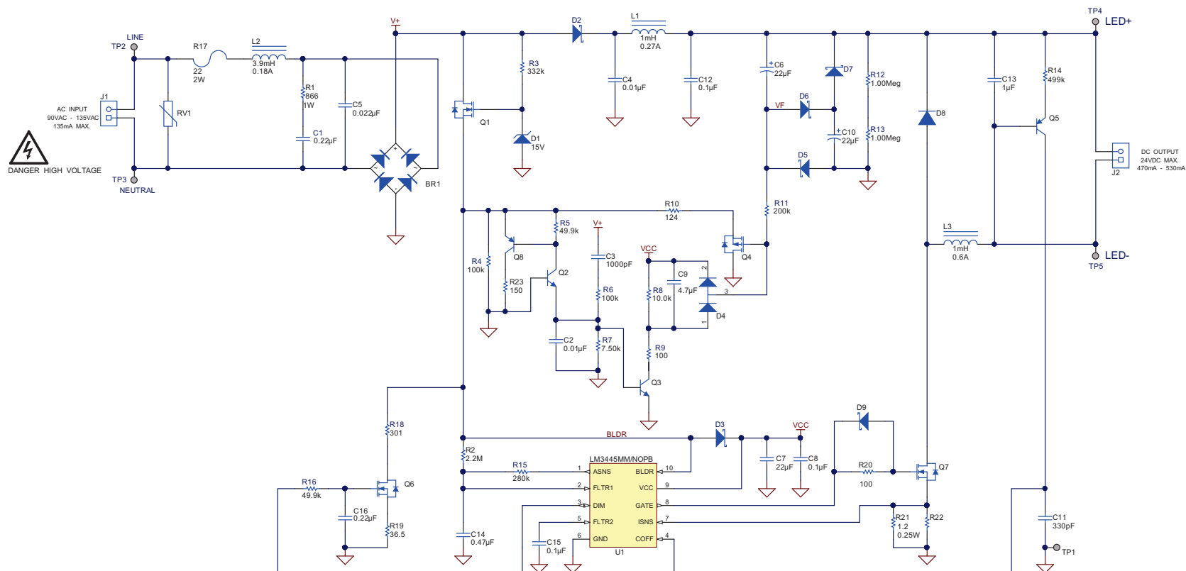
Figure 1. LM3445EVM-695 Schematic
