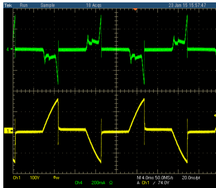
Figure 11. Lutron Trailing Edge DVELV-303P, Output = 150 mA, V_{LED} = 22 V
