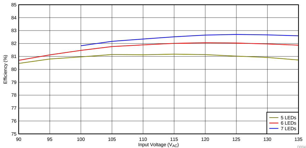
Figure 6. LM3445EVM-695 Efficiency
