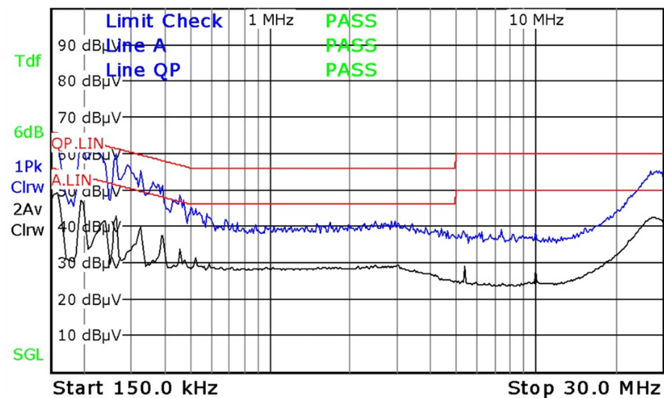
Figure 13. EMI Scan
