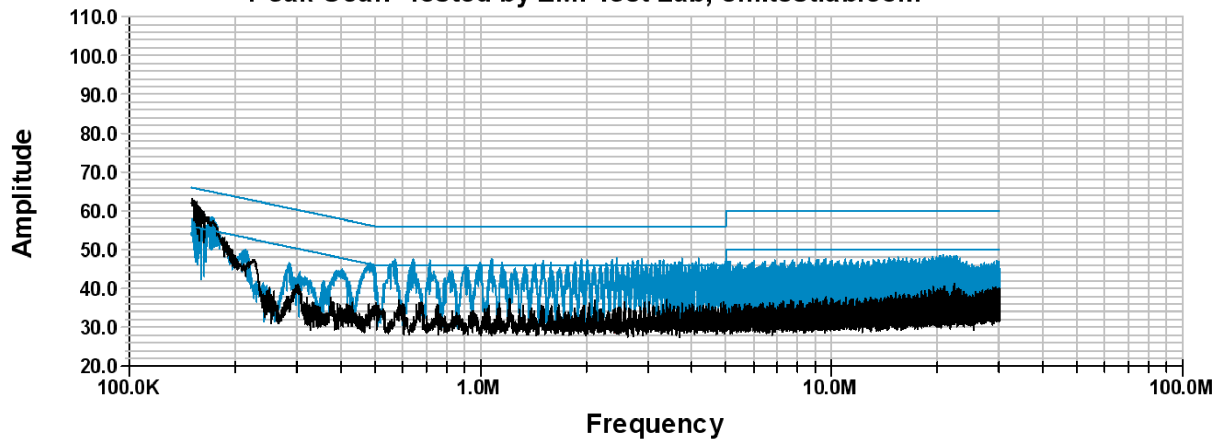
Figure 11. Conducted EMC. Line = Blue, Neutral = Black
