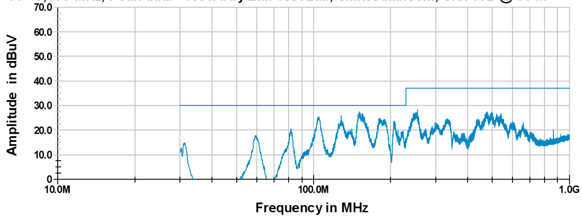
Figure 10. Radiated EMI
