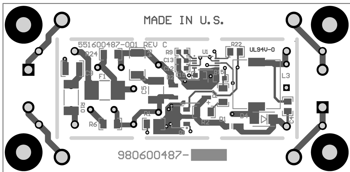
Figure 9. Bottom Layer
