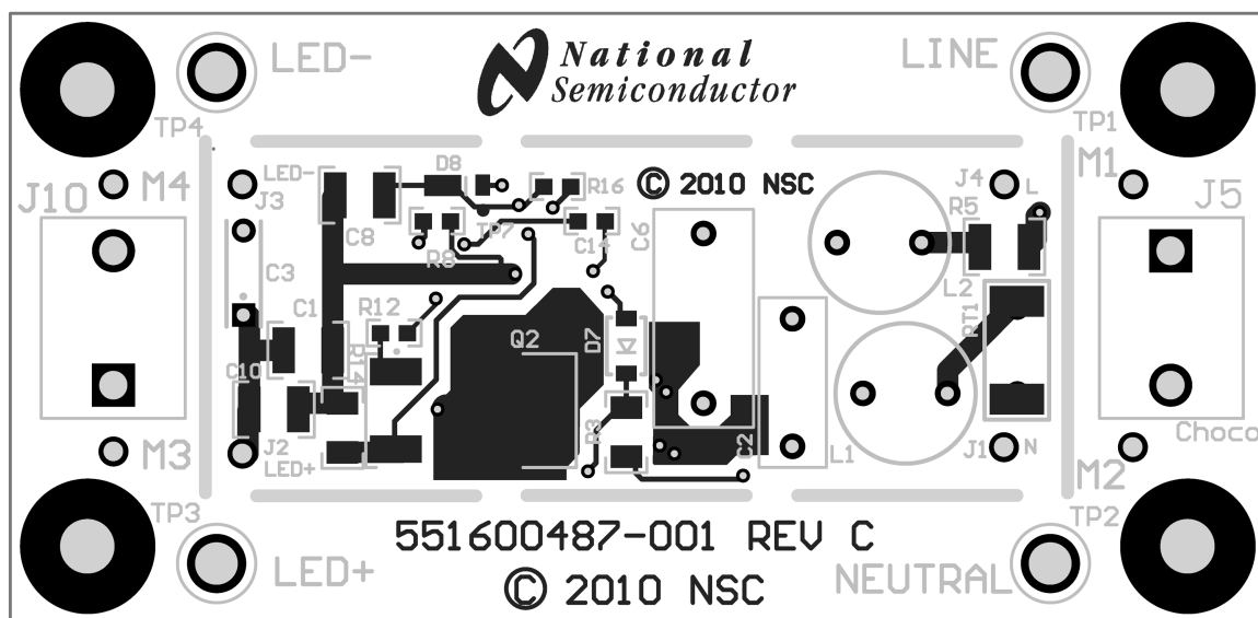
Figure 8. Top Layer
