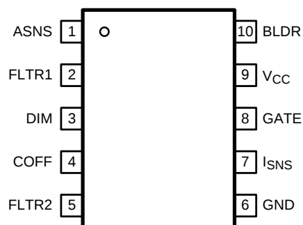
Figure 1. 10-Pin VSSOP
