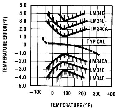
Figure 15. Temperature Error
