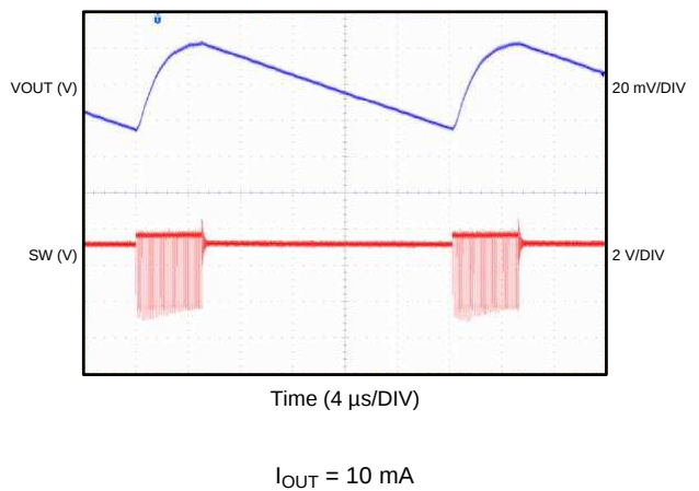
Figure 7. Output Voltage Ripple in ECO Mode
