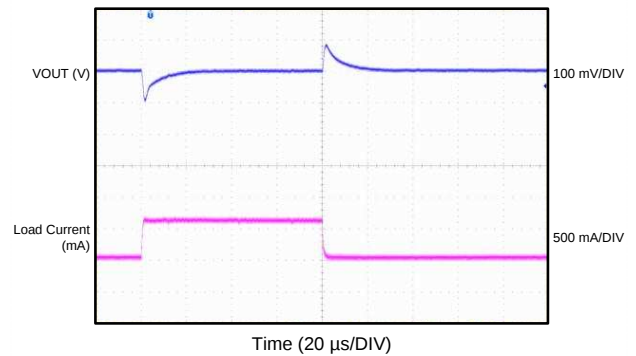
Figure 21. Load Transient Response
