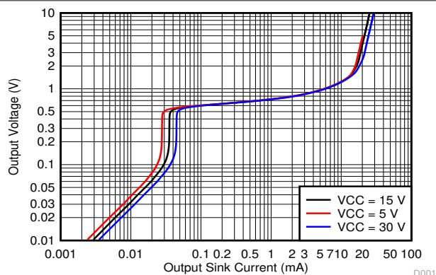
Figure 6-1. Output Sinking Characteristics
