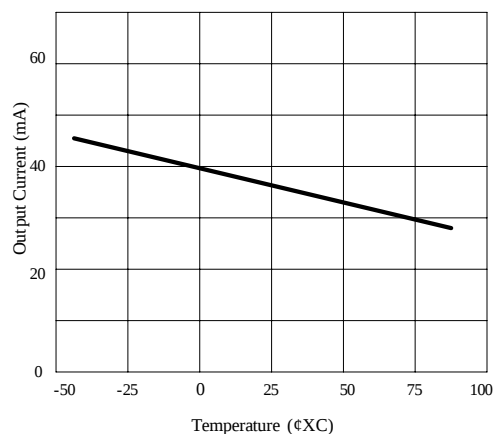
Fig.12 Current Limiting
