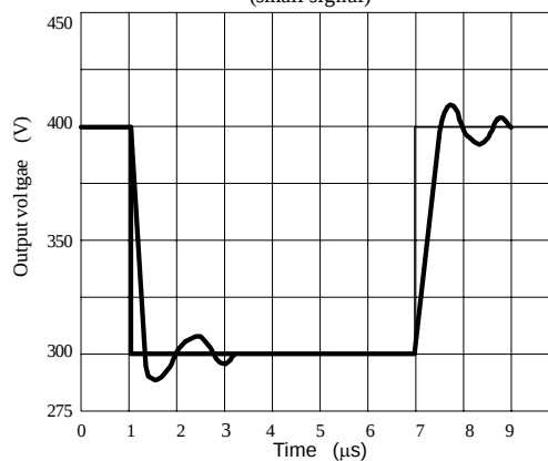
Fig.8 Voltage Follower pulse response (small signal)
