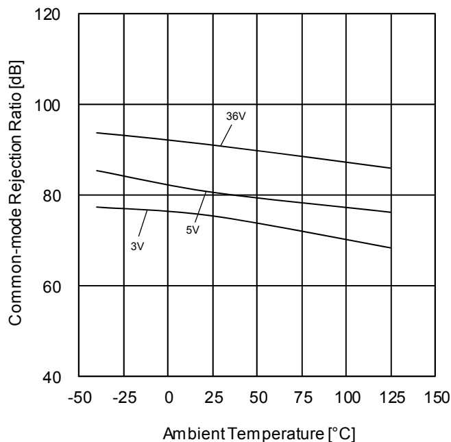
Figure 28. Common-mode Rejection Ratio vs Ambient Temperature
