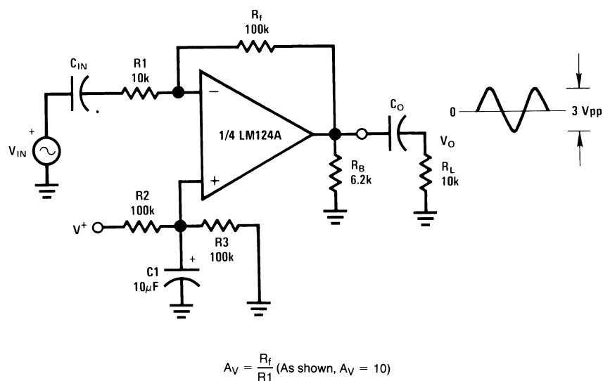
Figure 37. AC Coupled Inverting Amplifier
