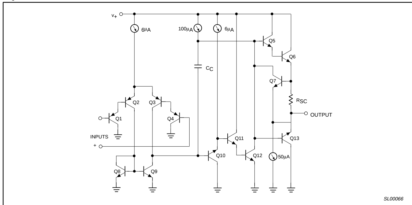
Figure 2. Equivalent Circuit
