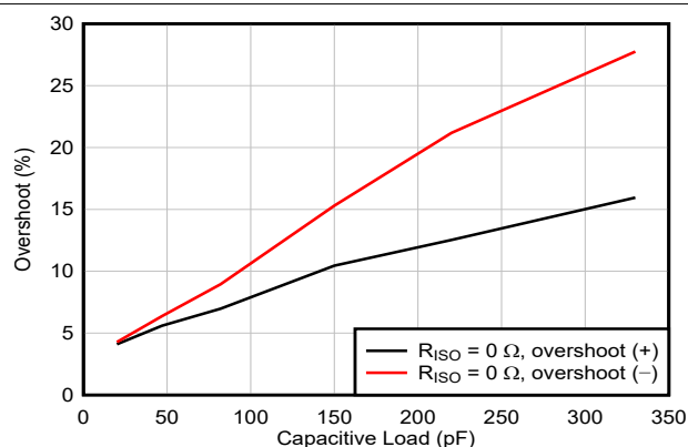
Figure 6-19. Small-Signal Overshoot vs Capacitive Load
