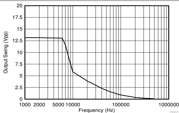
Figure 6-34. Maximum Output Swing vs. Frequency (VCC = 15 V)
