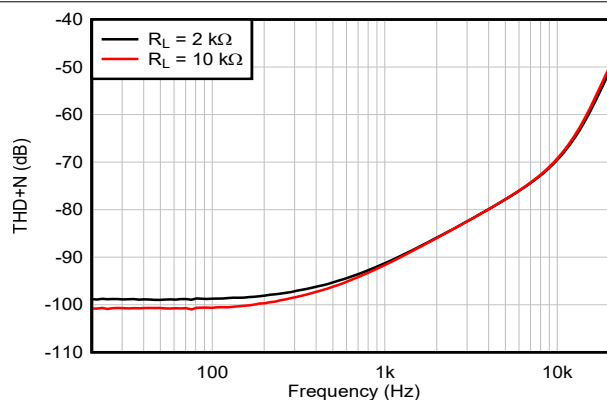
Figure 6-12. THD+N Ratio vs Frequency, G = 1 G = 1 , f = 1\text{ kHz} , BW = 80\text{ kHz} , V_{OUT} = 10\text{ V}_{PP} , R_L connected to V_-
