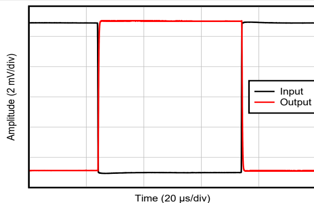
Figure 6-25. Small-Signal Step Response, G = -1
