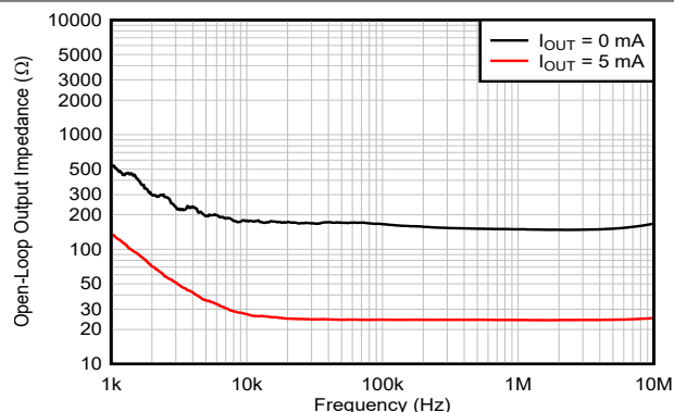
Figure 6-18. Open-Loop Output Impedance vs Frequency
