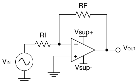
Figure 9-1. Application Schematic
