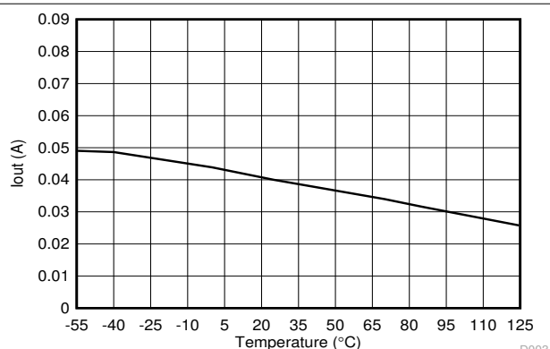
Figure 6-31. Source Current Limiting
