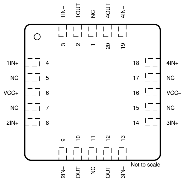
Figure 5-2. FK Package 20-Pin LCCC (Top View)
