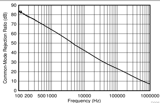
Figure 6-33. Common-Mode Rejection Ratio
