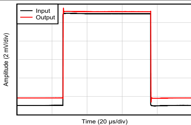
Figure 6-22. Overload Recovery (Positive Rail)
