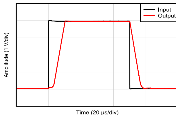
Figure 6-26. Large-Signal Step Response, G = 1
