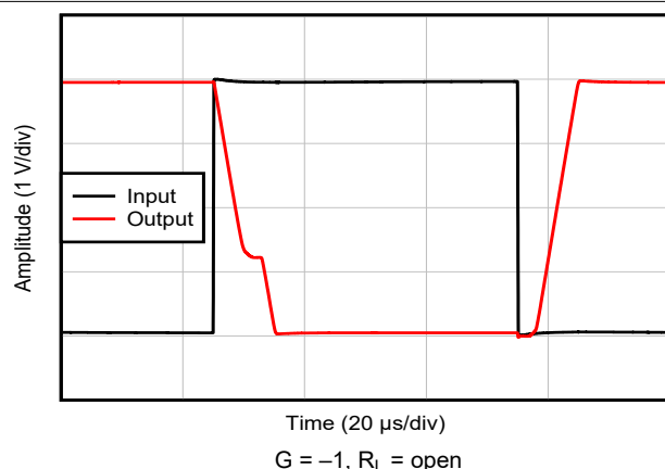
Figure 6-27. Large-Signal Step Response, G = -1
