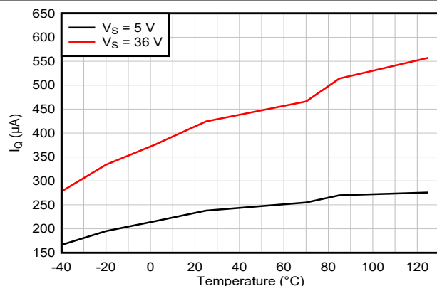
Figure 6-17. Quiescent Current vs Temperature
