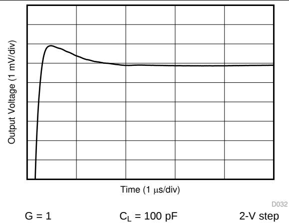
Figure 26. Large-Signal Settling Time (Positive)
