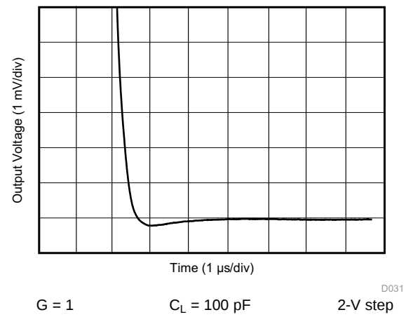
Figure 25. Large-Signal Settling Time (Negative)
