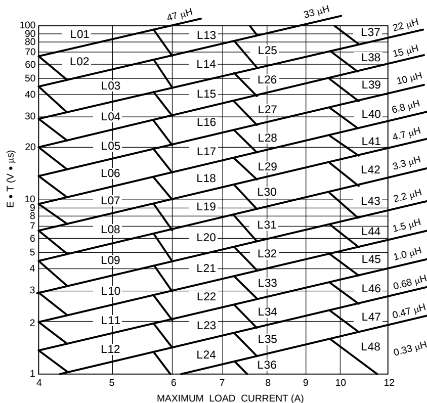
Figure 13. Inductor Nomograph
