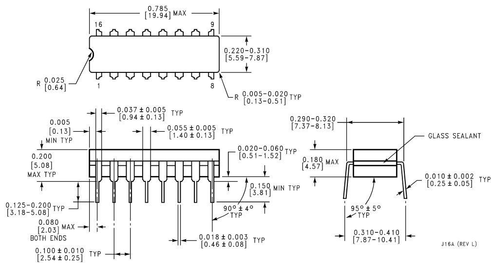
16-Lead Ceramic Dual-in-Line Package LM2990J-5.0-QML (5962-9571101QEA), LM2990J-12-QML (5962-9571001QEA), or LM2990J-15-QML (5962-9570901QEA), NS Package Number J16A
