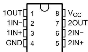
D, DGK, JG, P, PS, or PW 8-Pin SOIC, VSSOP, CDIP, PDIP, SO, or TSSOP Top View
