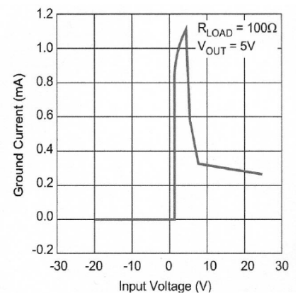
LM29150 Ground Current vs. Input Voltage
