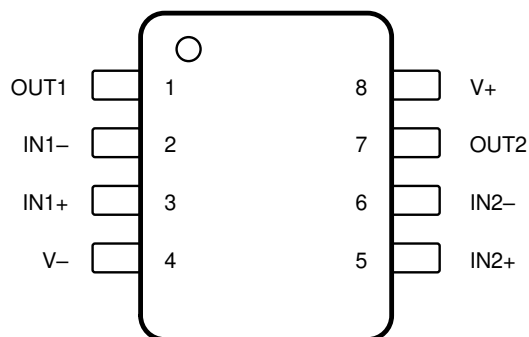
Figure 6-1. D, DDF, DGK, P, PS, PW, and JG Package
