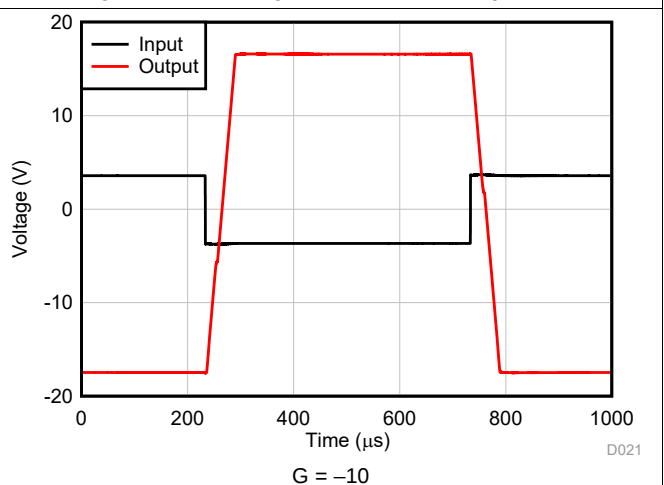
Figure 28. Overload Recovery
