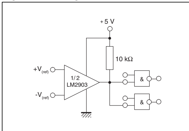
Figure 10. Driving TTL
