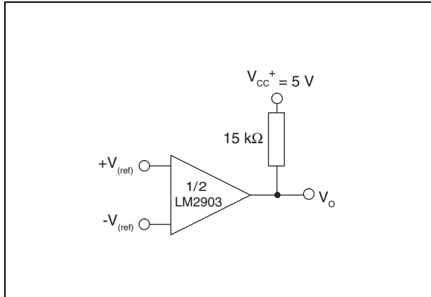
Figure 7. Basic comparator
