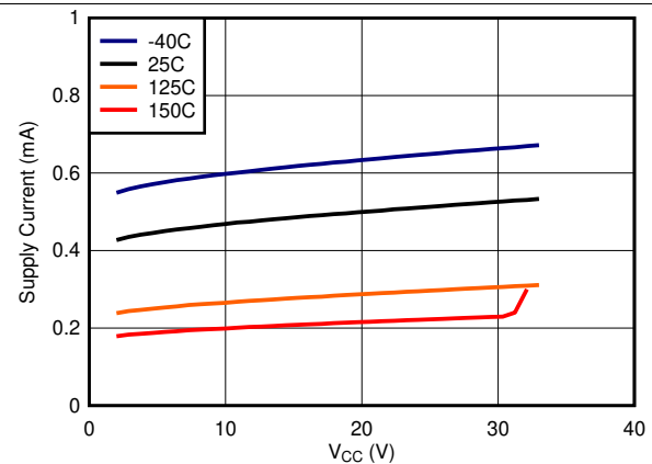
Figure 2. Supply Current vs. Supply Voltage LM2903E-Q1 Only
