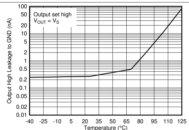
Figure 30. Output High Leakage Current vs. Temperature at 36V
