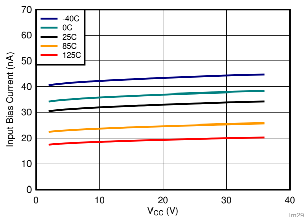
Figure 3. Input Bias Current vs. Supply Voltage
