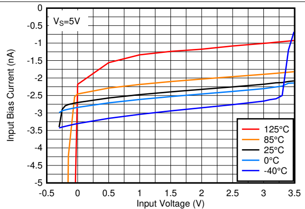
Figure 22. Input Bias Current vs. Input Voltage at 5V
