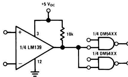
Figure 8. Driving TTL
