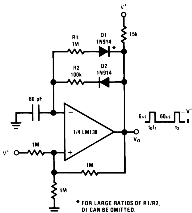
Figure 14. Pulse Generator
