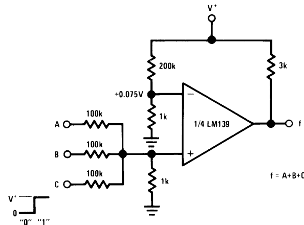
Figure 10. OR Gate
