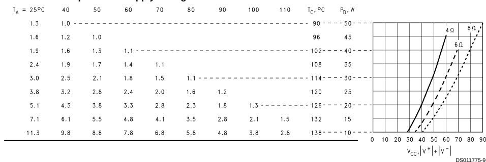
Max Heatsink Thermal Resistance ( ^{\circ}\text{C}/\text{W} ) at the Specified Ambient Temperature ( ^{\circ}\text{C} ) Maximum Power Dissipation vs Supply Voltage
