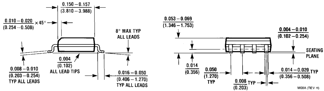
SO Package (M) NS Package Number M08A
