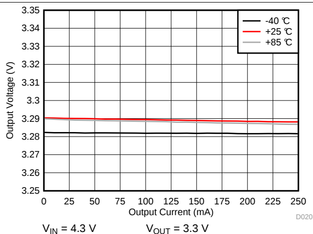
Figure 8. Load Regulation for OUT+
