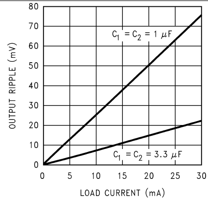
Figure 8. Output Ripple vs Load Current
